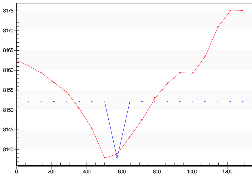
Figure 4-2: DEM Elevation Profile Plot
